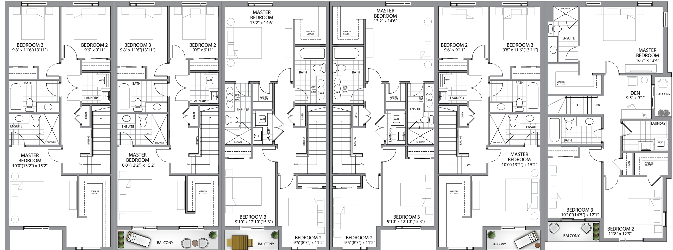
UNIT 6-S2/MB 2nd Floor: 971 sq. ft.
