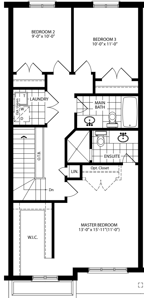
Second Floor Interior Unit • S2 Layout applies to units: 72, 73, 74 & 75
