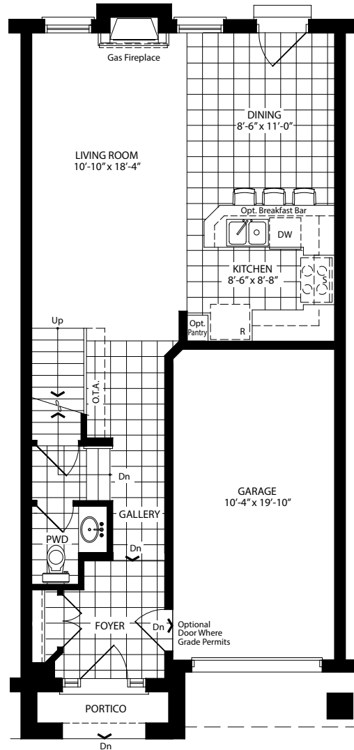
Opt Ground Floor • G2
