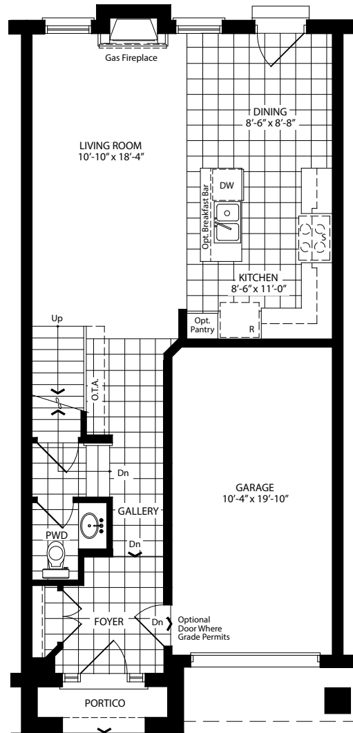
Ground Floor • G1
